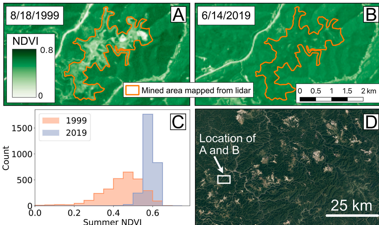
Fig. 10. A demonstration of the influence of MTR/VF mining on vegetation loss and recovery. A) In this Landsat image, the normalized difference vegetation index (NDVI; a spectral measure of greenness) is lower within the mined polygon (mapped by Reed and Kite (2020)) than in the surrounding forest, indicating that mining has reduced vegetation cover. B) 20 years later, NDVI is similar between the mined polygon and its surroundings. C) The distribution of NDVI within the mined polygon has shifted towards higher values and become narrower over the 20-year period. D) Zooming out illustrates the striking differences in vegetation cover between active mines and the surrounding landscape (image from Google Earth).
